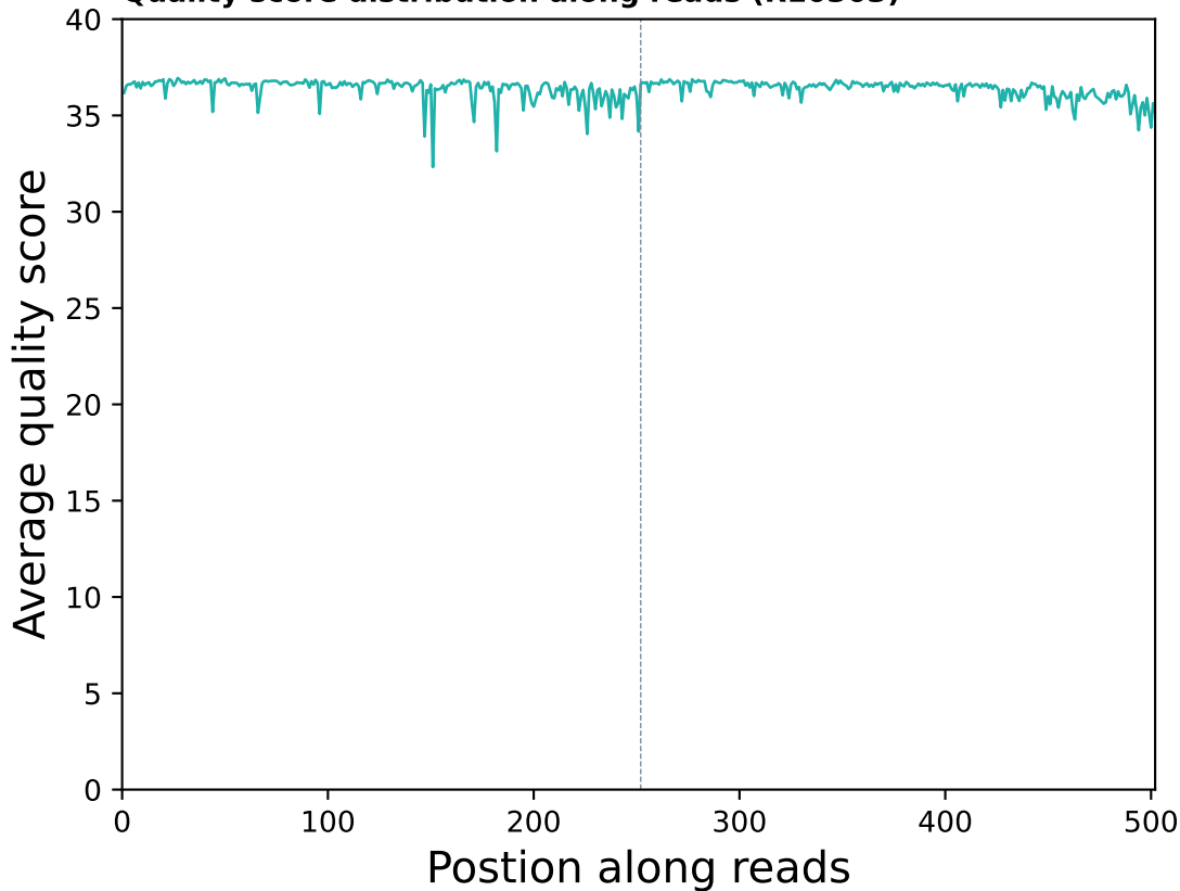
Quality score distribution along reads (R10303)
